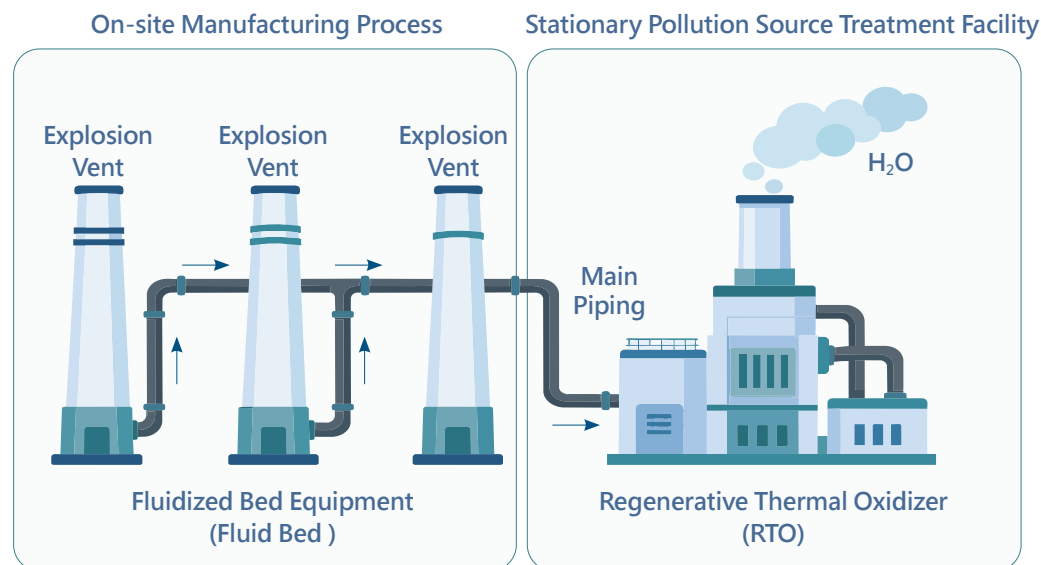
Flowchart of Organic Solvent Exhaust Treatment Process
